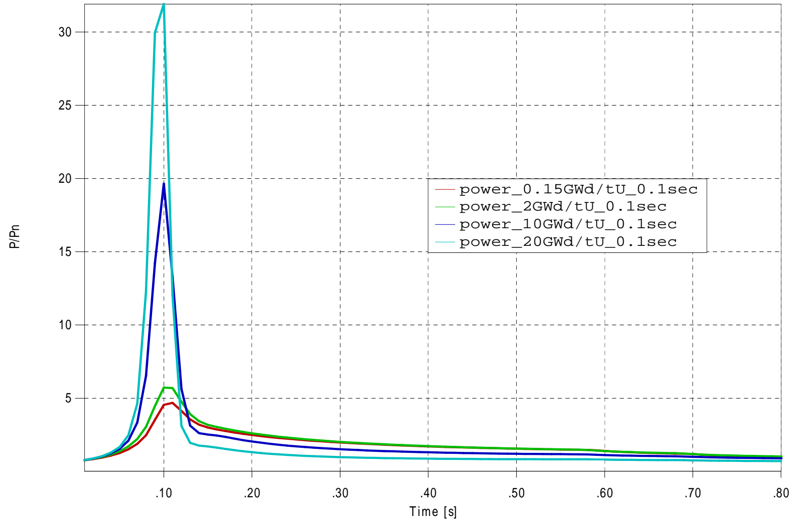
Nuclear power rate
